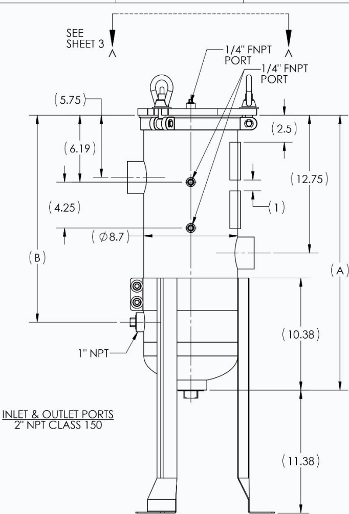
REFERENCE ENGINEERING DRAWING 21132
